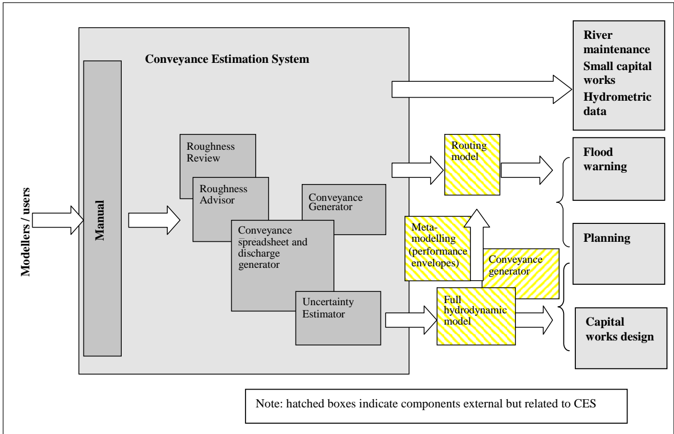
Figure 3 Components of the Conveyance Estimation System
